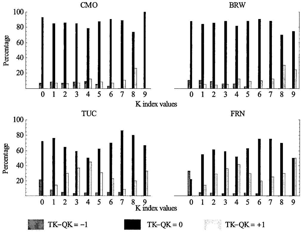
Figure 22 - Performance of the new USGS K index algorithm based on K index category.
